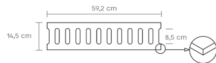
OVERFLOW GRILLE
