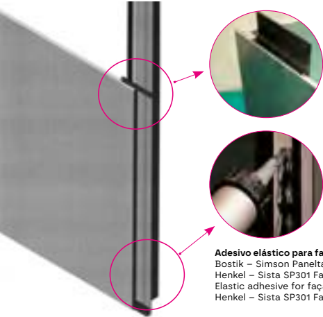
FACHADA COLADA FACADES USING ADHESIVES FAÇADE COLLÉE FACHADA PEGADA
